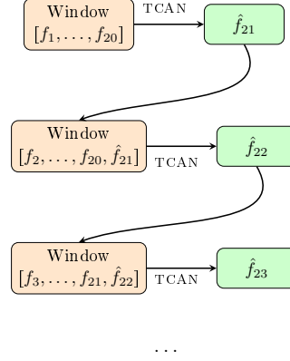
Figure 4.5: Autoregressive rollout process: each TCAN call maps a window of previous fields to one predicted field. In this example, the model first predicts f_{21} from the window [f_1, \dots, f_{20}] , then uses the updated window [f_2, \dots, f_{20}, f_{21}] to predict f_{22} , and so on.
